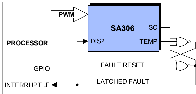
Figure 6. External Fault Latch Circuit
