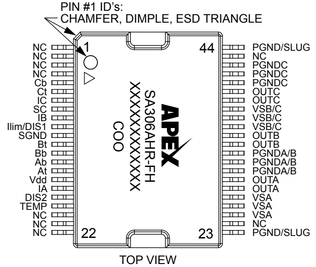
Figure 3B. External Connections 44-pin HSOP, Slug-Down, HR Pkg.
