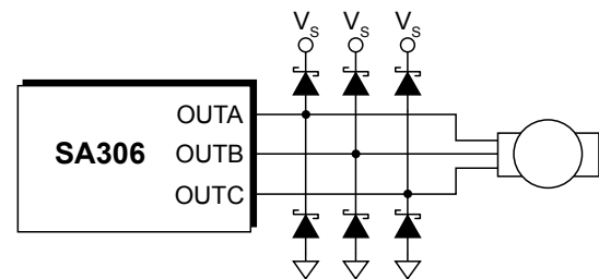
Figure 9. Schottky Diodes
