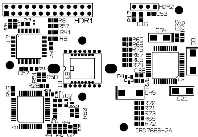
SILKSCREEN - TOP
