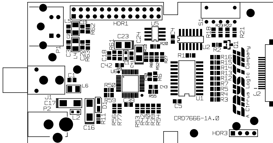
SILKSCREEN - TOP
